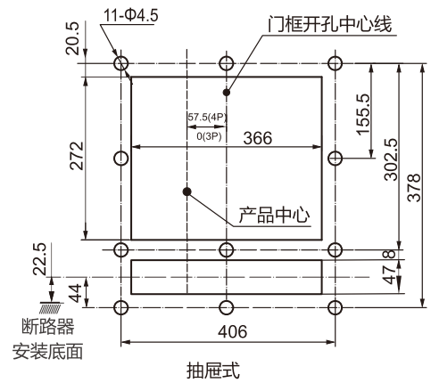
RDW5-4000H抽屉式断路器面板开孔尺寸
