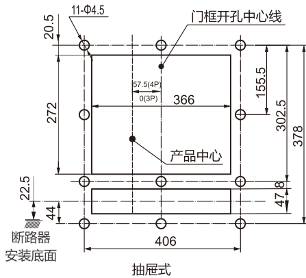
RDW5-3200H抽屉式断路器面板开孔尺寸
